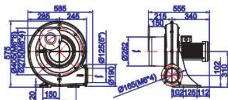
TB100-1 / TB100-2
