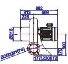
TB200-15 / TB200-20
