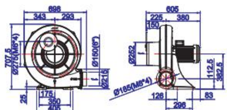
TB150-5
