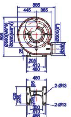
TB200-15 / TB200-20
