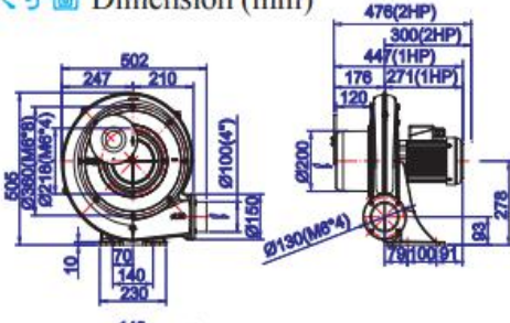
TB100-1 / TB100-2
